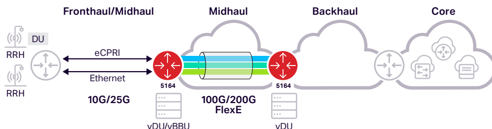
Figure 1. Cloud-RAN network application
