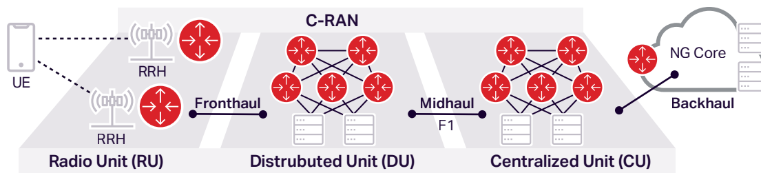
Figure 2. 5G NR RAN architecture
