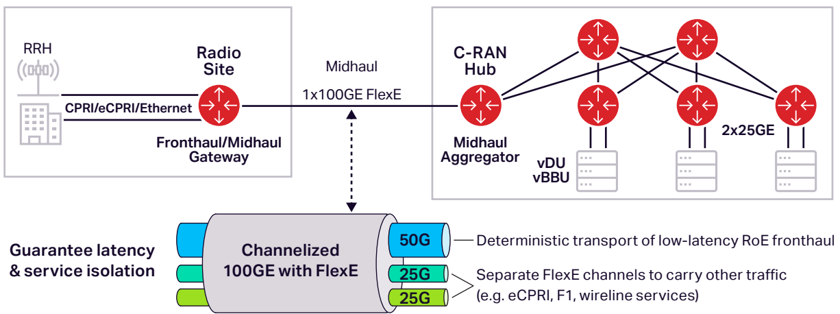
Figure 4. 5164 Channelized FlexE
