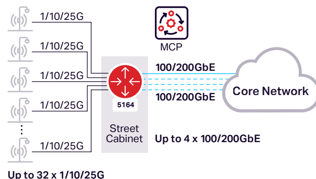
Figure 3. 5164 Router outside service and aggregation
