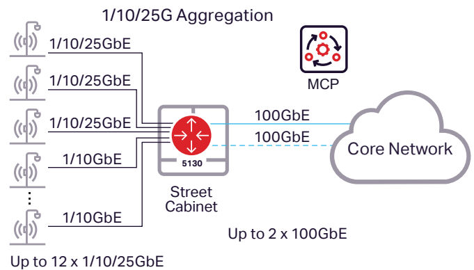
Figure 3. 5130 Router outside service and aggregation
