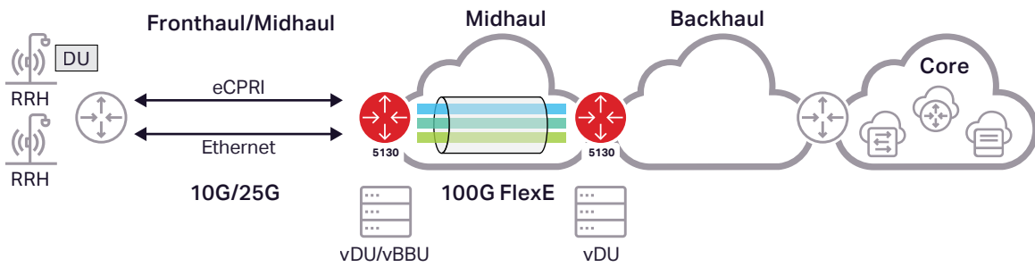
Figure 1. Cloud-RAN network application
